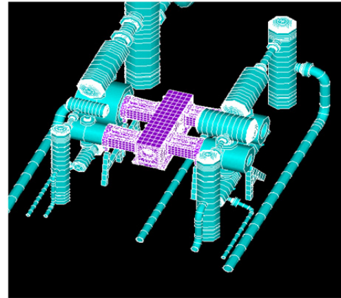
Figure 3.1 Accurate FE modeling, including “super-element” compressor frame
