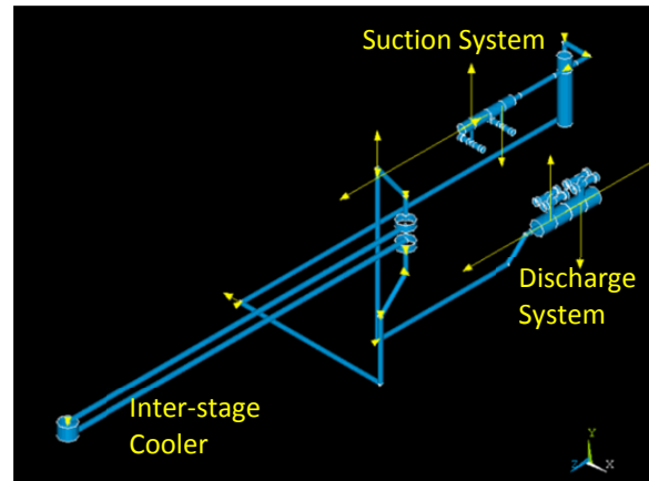
Figure 2.1 Pulsation forces in an inter-stage system, using BETA's Time Domain acoustical solver
