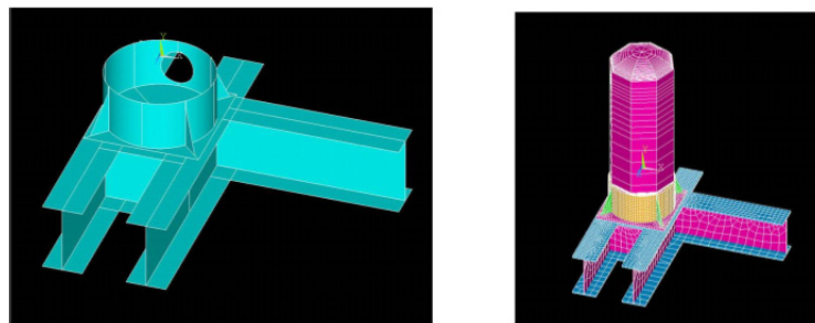
Figure 3.2 FEA includes 3-D modeling of scrubber bases required for accurate boundary condition assumptions
