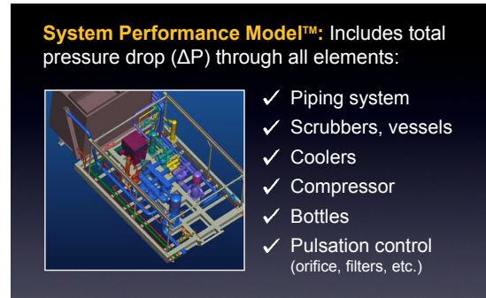
Figure 1.1 System Performance Model (SPM) for reciprocating compressor design
