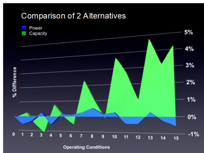
Figure 1.3 Compressor Design Optimization using SPM tool
