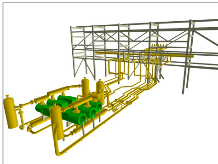
Examples where an integrated approach is used to mitigate vibration risks in the piping system, compressor and pump skids, offshore & onshore foundations, and elevated structural supports.
